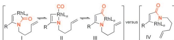
Scheme 2. Proposed mechanism of the [2+2+2] cycloaddition.
